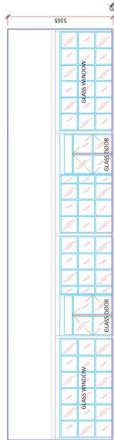
20 x 10 m TENT LAYOUT, WITH 20 x 3 m WOODEN TERRACE
